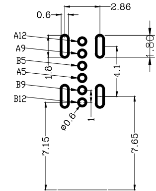
RECOMMENDED P.C.B. LAYOUT TOLERANCE UNSPECIFIED ±0.05mm
