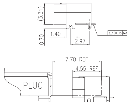
MATING INTERFACE
